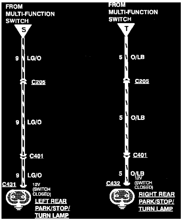
Turn/Stop/Hazard Lamps
