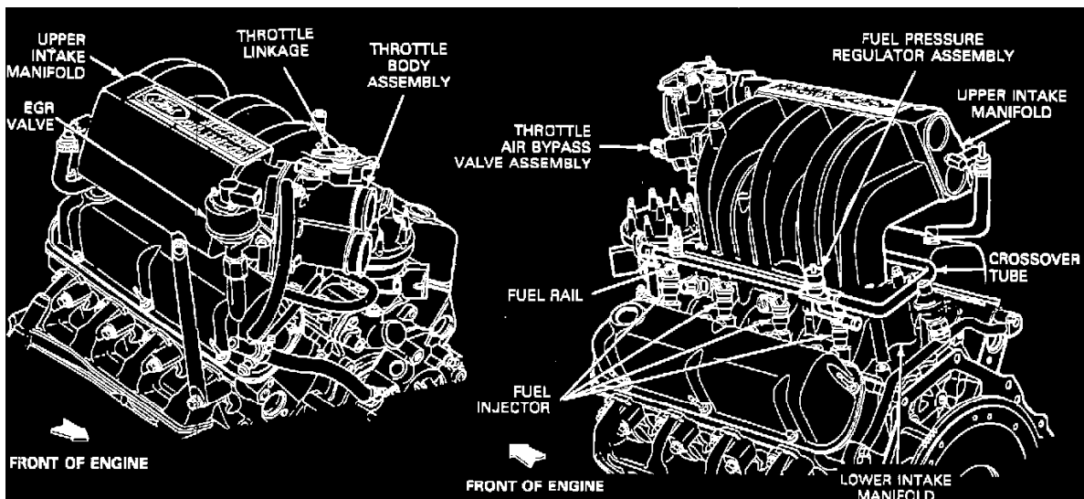
Component Location
