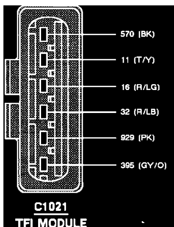
Thick Film Ignition Module Connector Pinout
