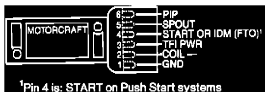
Remote Mounted TFI-IV Ignition Module
